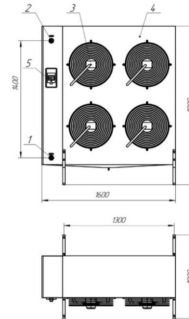
Carbon dioxide atmospheric gasifier GU500A. Dimensional drawing.
